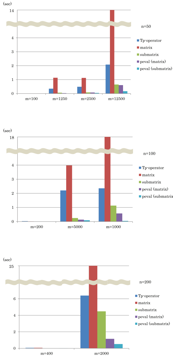
Fig. 4. Comparison of runtime for fixpoint computation
